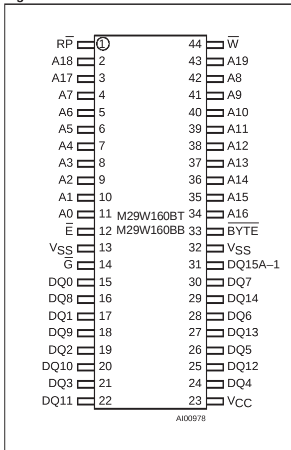
Figure 3. SO Connections
